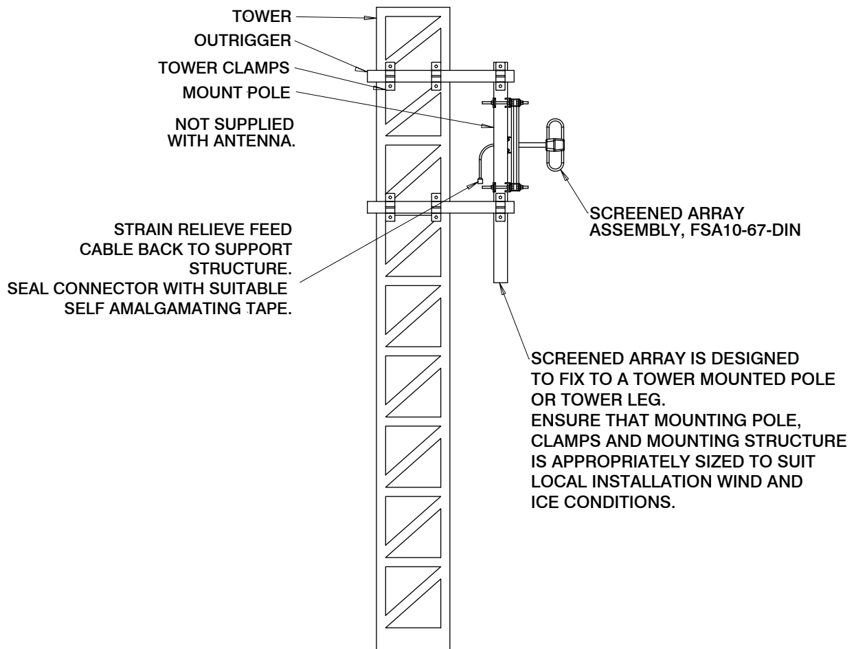
TYPICAL INSTALLATION SIDE VIEW
