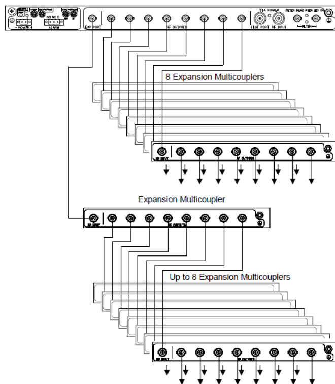
Fig 5 - Up to 128 equal level RF Outputs
