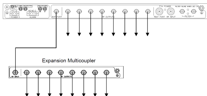
Fig 3 - Up to 16 equal level RF Outputs
