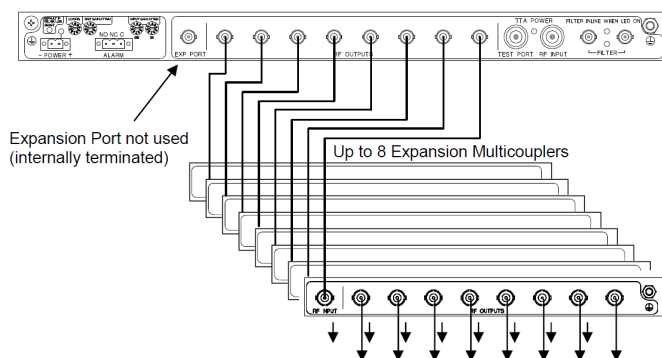
Fig 4 - Up to 64 equal level RF Outputs
